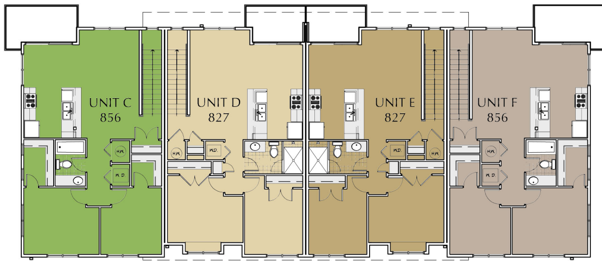
2ND LEVEL PLAN 1/16" = 1'-0" NORTH
