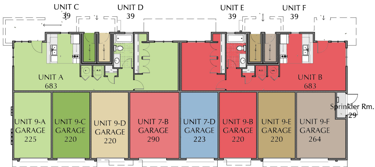
GROUND LEVEL PLAN 1/16" = 1'-0" NORTH
